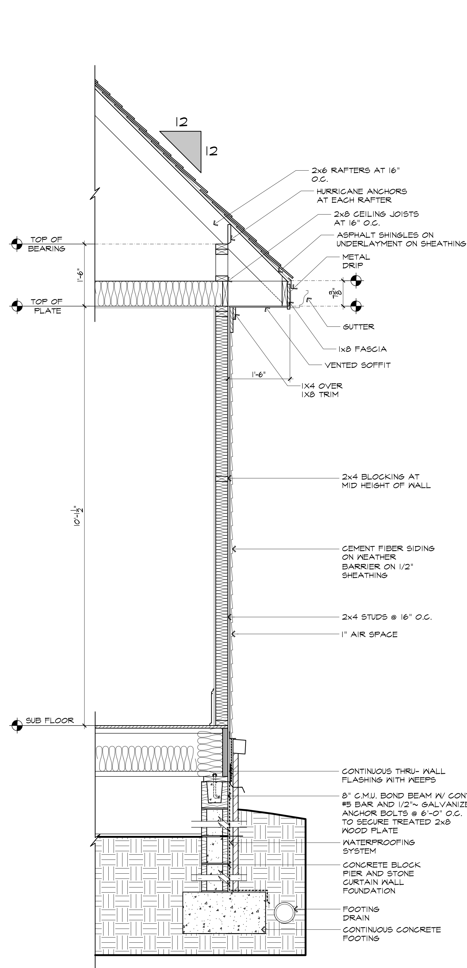
TYPICAL STORY WALL SECTION
